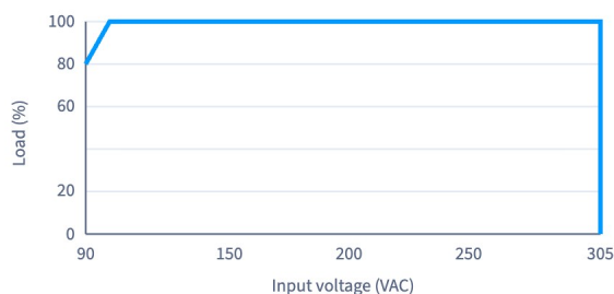
Load vs input voltage (60 Hz)
